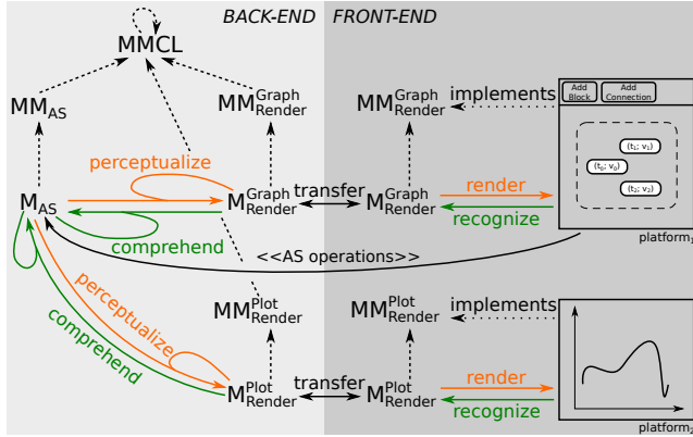
Figure 13. Approach with multiple MM_{Render} models.
