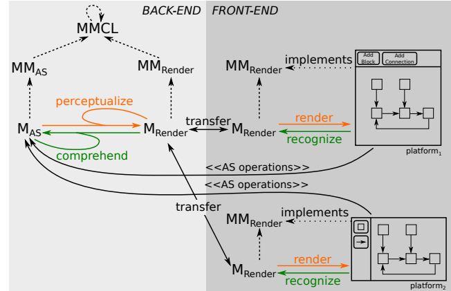
Figure 12. Approach with multiple GUI front-ends.
