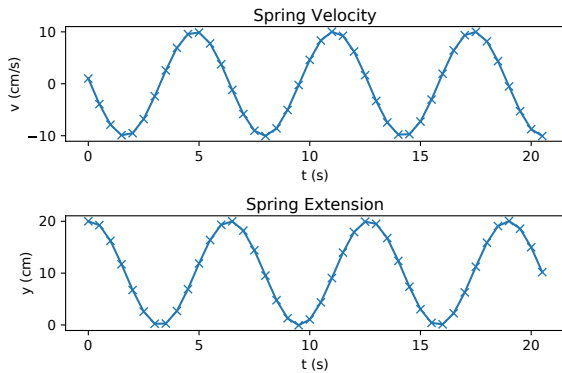
Figure 3. Plotted trace of the CBD model in Figure 2, with k = 1 , m = 1kg , y_0 = 20cm , v_0 = 1 \frac{cm}{s} , and g = 10 \frac{cm}{s^2} .
