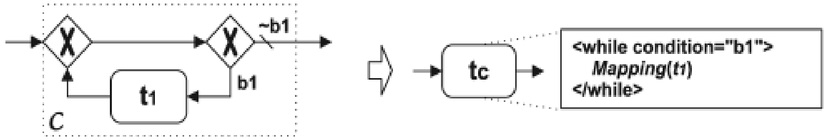
( e ) WHILE-pattern
