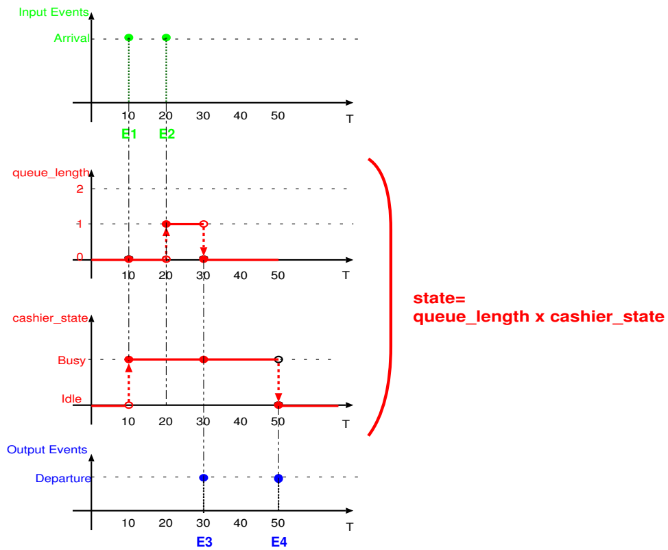
Figure 2: Queuing system state trajectory
