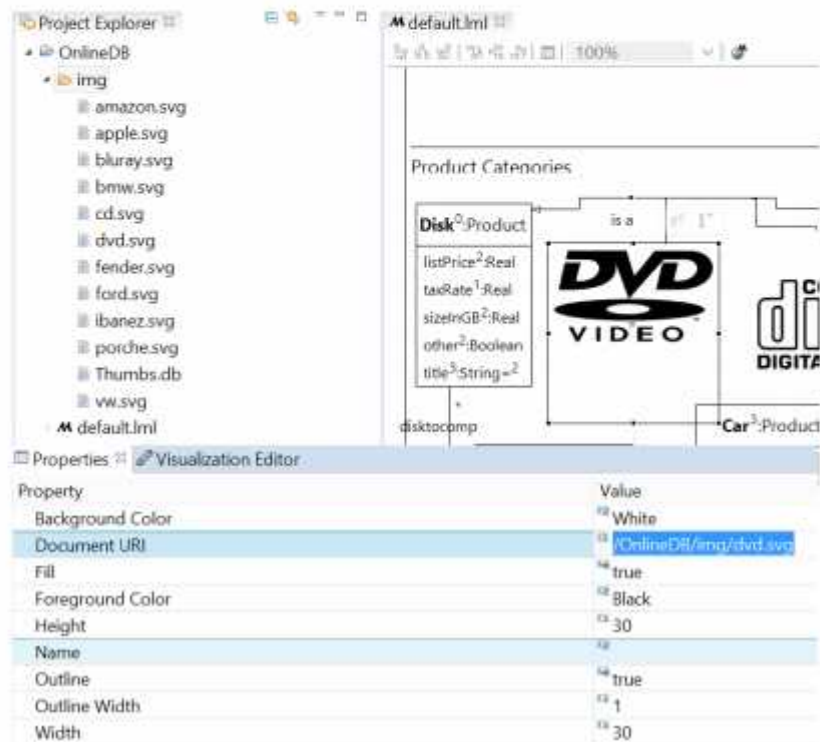
Figure 9: SVG Properties
