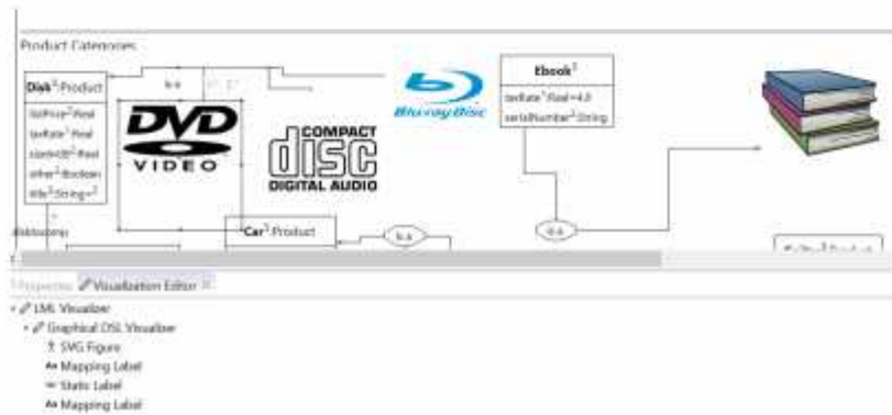
Figure 8: DVD Visualization
