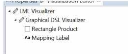
Figure 5: Product Visualization
