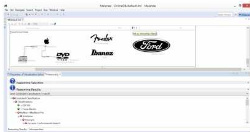
Figure 14: Error Mac
