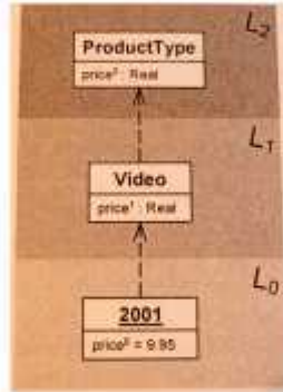
Figure 3: Deep Instantiation example in the above picture
