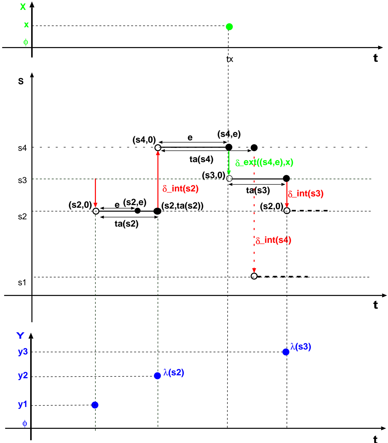
Figure 1: State Trajectory of a DEVS-specified Model
