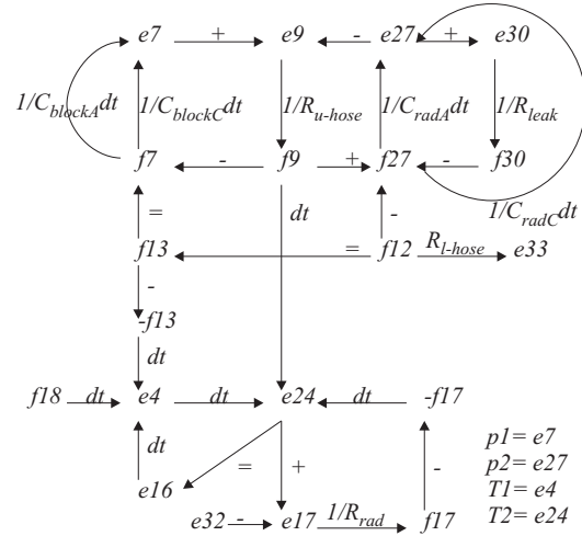
Figure 7: TCG of the automotive cooling system.
