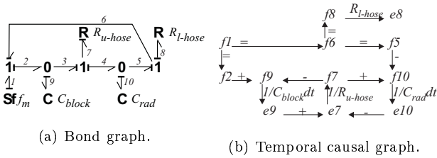
Figure 1: Hydraulics of an automobile cooling system.
