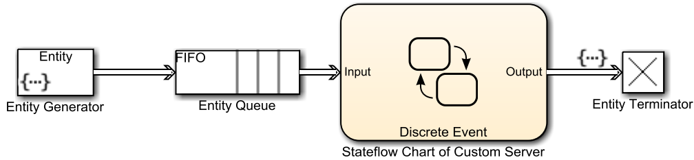
Figure 3: Example custom event actions of Entity Generator block and Entity Server block.
