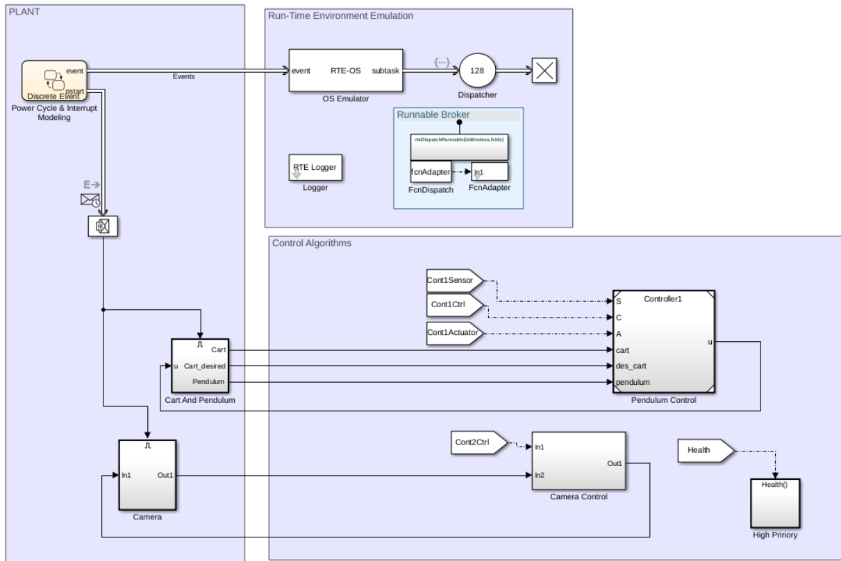
Figure 7: Application example of real-time operating system.
