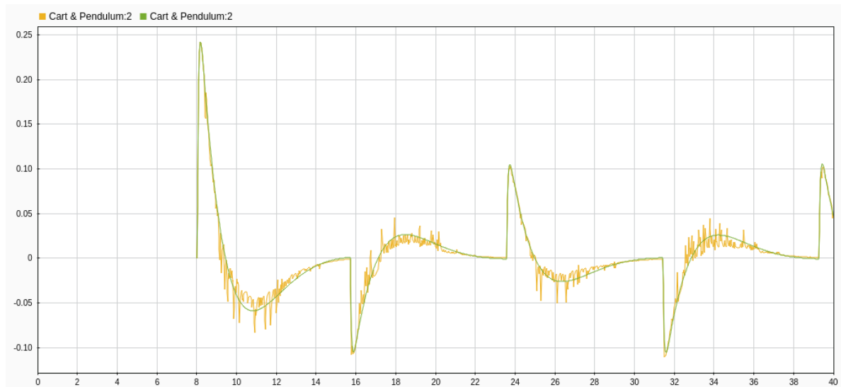
Figure 9: Results of running the simulation that show deviation of the pendulum from vertical. The yellow line shows the pendulum position that is influenced by scheduling jitter on a single-core system. The green line shows the elimination of jitter by using a two core system.
