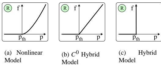
Figure 2: Levels of Abstraction of a Cylinder End-stop
