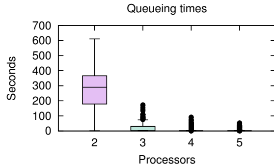
Figure 10: Boxplot of queueing times for varying number of active processors.
