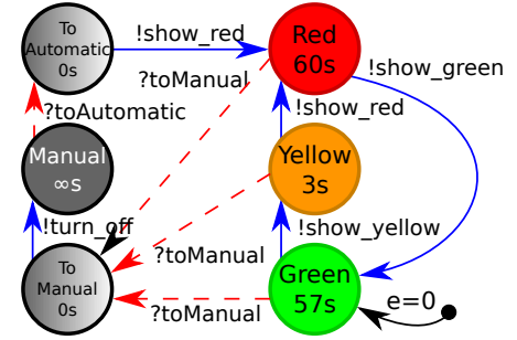
Figure 8: Model generating trace in Figure 7.
