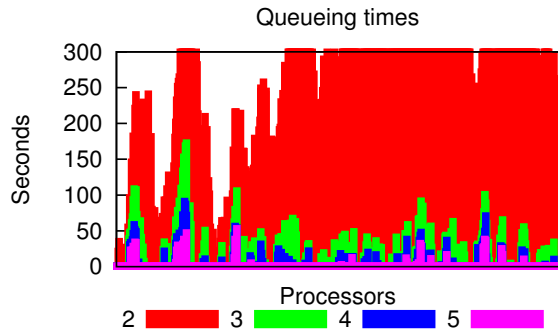
Figure 9: Evolution of queueing times for sub-sequent customers.
