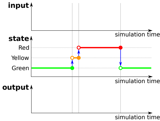
Figure 1: Trace of the autonomous traffic light.
