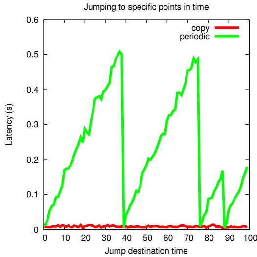
Figure 6: Jump latency for copy and periodic state saving.
