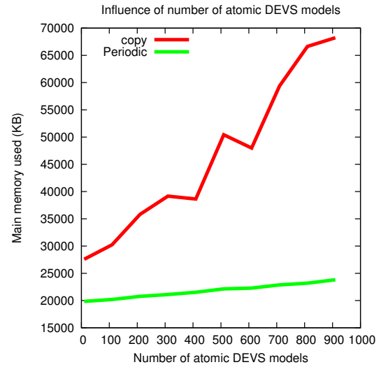
Figure 7: Influence of number of atomic models on memory consumption.
