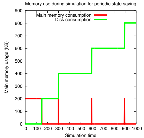
Figure 5: Memory use of periodic state saving.
