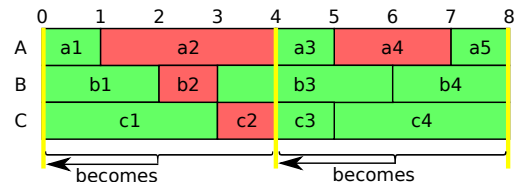
Figure 2: Overview of periodic state saving approach. Green states (light) are stored, red (dark) states are not. Yellow lines indicate a point at which a snapshot is made.
