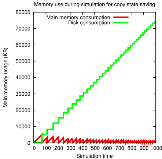
Figure 4: Memory use of copy state saving.
