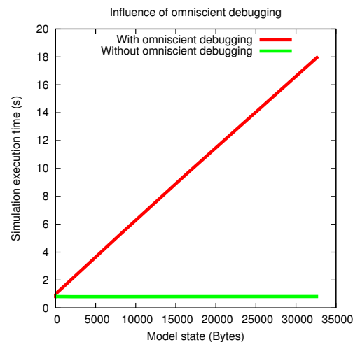
Figure 1: Overhead of omniscient debugging in forward simulation.
