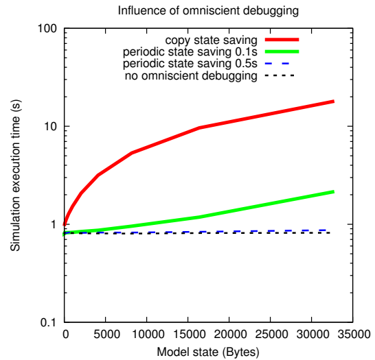
Figure 3: Overhead of omniscient debugging in function of state size (logarithmic scale).
